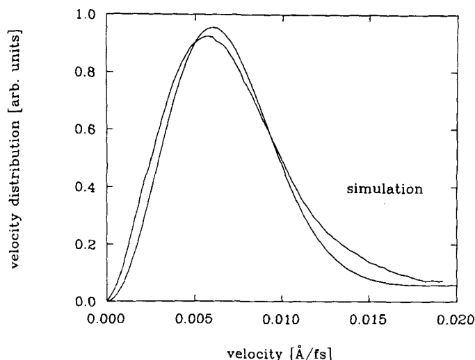
Figure 12 Comparison of the velocity distribution (at time t = 917 fs) resulting from a simulation of the photosynthetic reaction center and of the average Maxwell distribution evaluated according to Equation (18) for all reaction center atoms.
